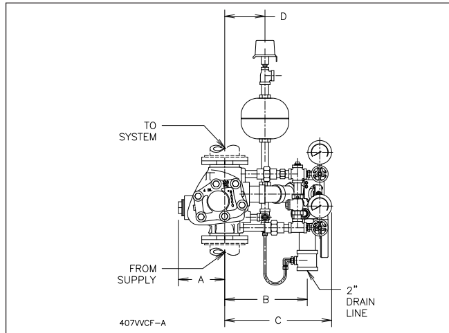
Vertical Variable Trim - Front Elevation
