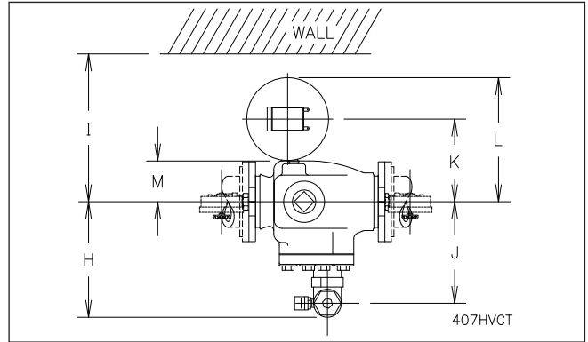
Horizontal Variable Trim - Top View
