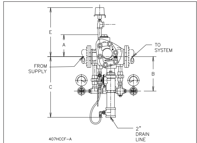
Horizontal Constant Trim - Front Elevation
