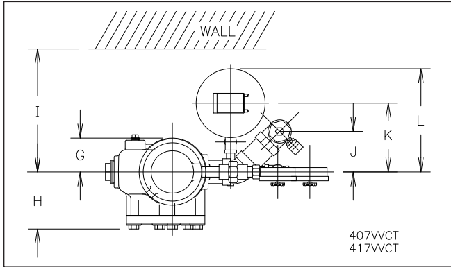
Vertical Variable Trim - Top View
