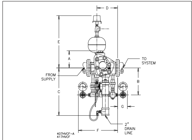
Horizontal Variable Trim - Front Elevation
