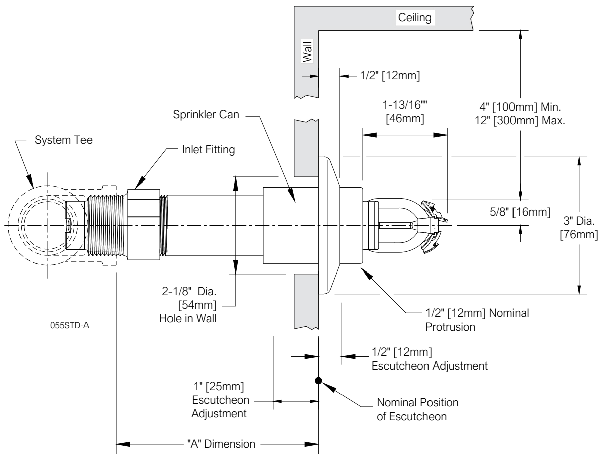
DH80 DRY HSW SPRINKLER, STANDARD ESCUTCHEON
