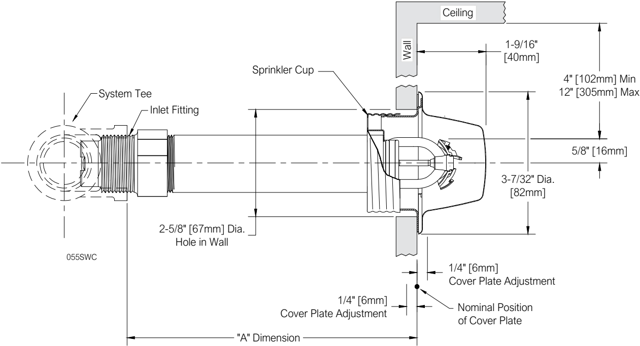
DH80 DRY HSW SPRINKLER, SWC CONCEALED COVER PLATE
