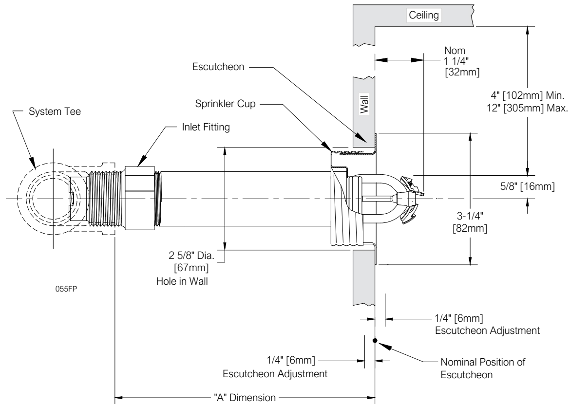
DH80 DRY HSW SPRINKLER, FP RECESSED ESCUTCHEON
